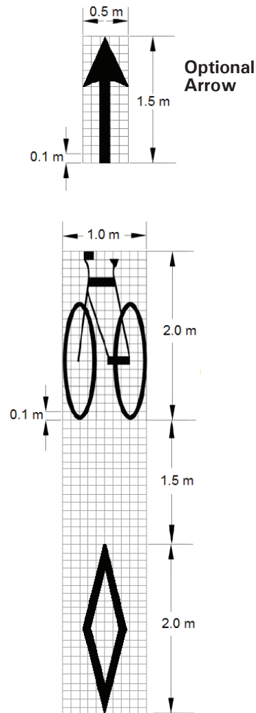
Figure 4.83 – Bicycle Lane Pavement Markings
