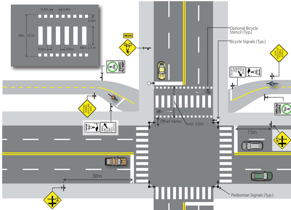
Figure 4.102 – Combined Pedestrian and Cyclist Crossside (Signalized Example)
