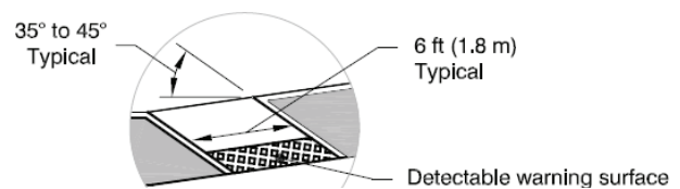
Figure 5.10 – Tapered Ramp Example
